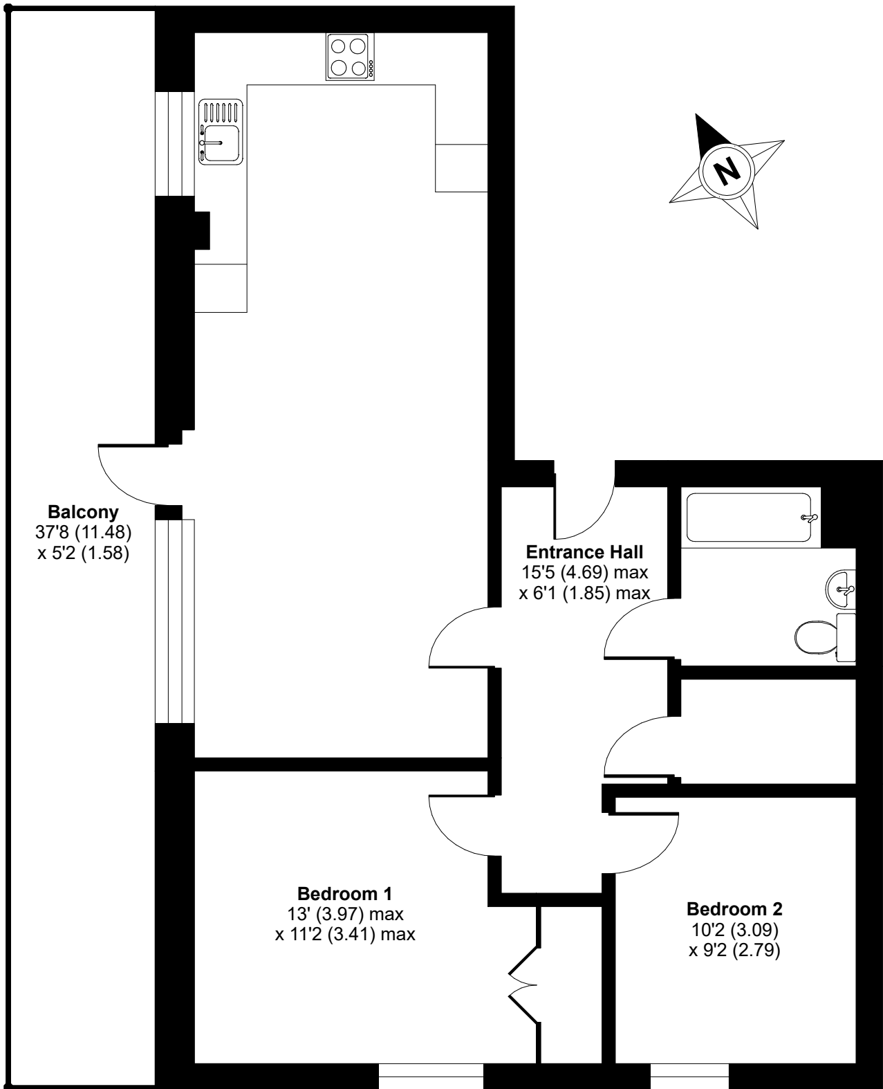
SECOND FLOOR
