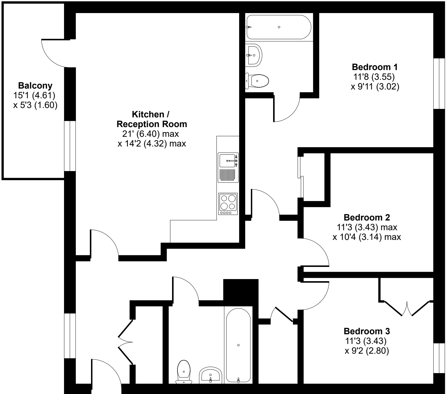
FIRST FLOOR
